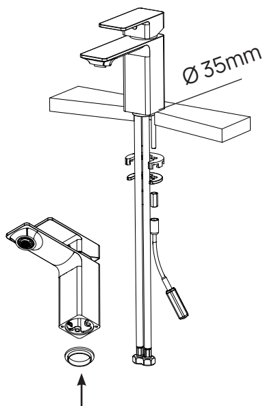
Montering uten base plate
